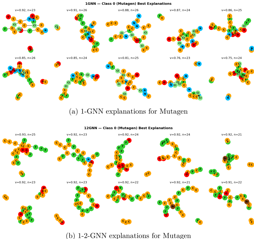
Figure 1: Top-ranked GIN-Graph explanations on MUTAG class 0 (Mutagen). The 1-GNN repeatedly produces mixed C/N/O scaffolds with scattered halogens, whereas the 1-2-GNN collapses onto narrower fluorine- and bromine-heavy prototype families. Node colours indicate atom types (see Figure 3).
