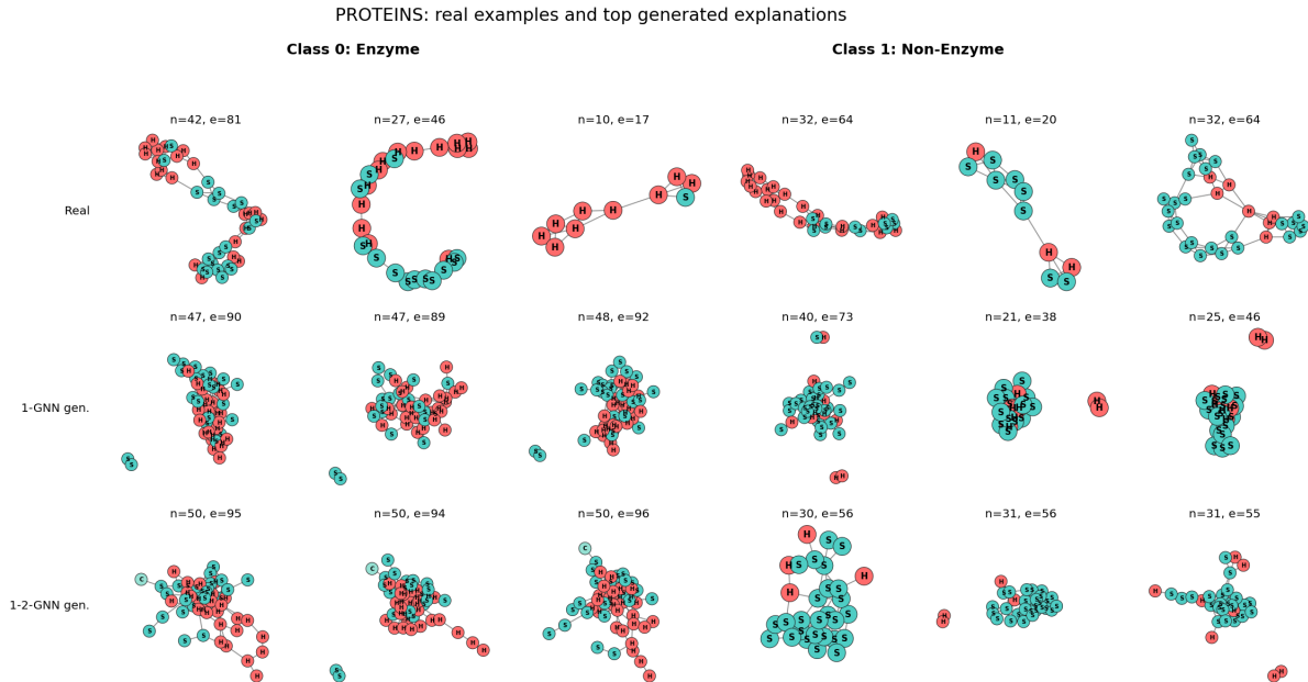
Figure 6: Illustrative PROTEINS examples. Each row shows three graphs from one source: real dataset graphs, top-ranked saved 1-GNN explanations, or top-ranked saved 1-2-GNN explanations. The generated examples make the population-level shifts easier to see, but they are not used as standalone evidence.
