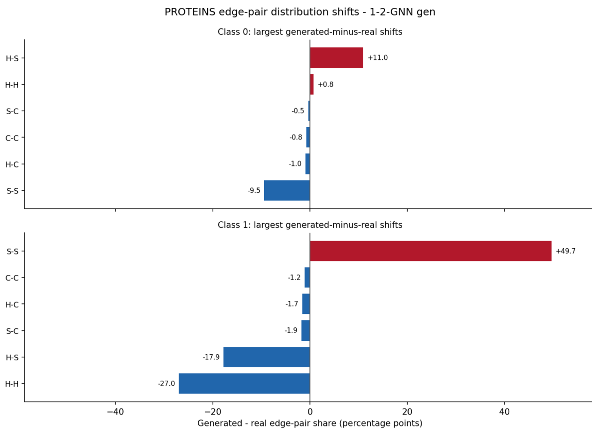
Figure 7: PROTEINS edge-type co-occurrence fingerprint for the 1-2-GNN generator. Bars show the largest generated-minus-real changes in unordered secondary-structure edge-pair shares, in percentage points, over 1000 generated graphs per class. Positive bars are over-produced by the generator; negative bars are under-produced.
