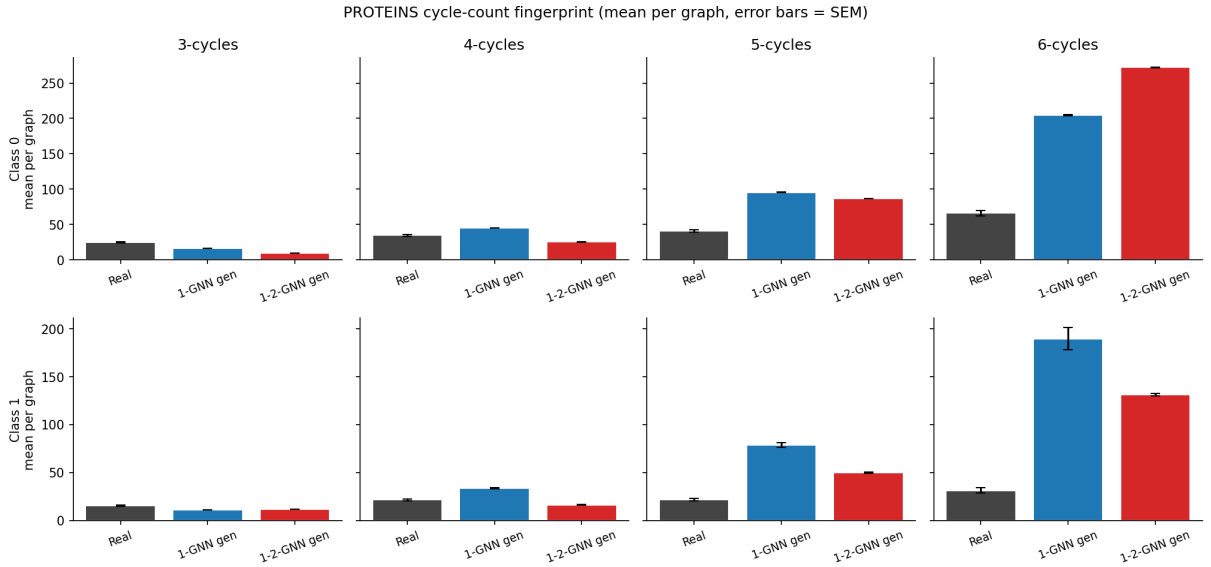
Figure 8: PROTEINS simple-cycle counts per graph, aggregated over 1000 generated graphs per cell. Error bars are the standard error of the mean. Both generators over-produce 5- and 6-cycles relative to real; the strongest differences appear in the 6-cycle panels, with the 1-2-GNN highest in class 0 and the 1-GNN highest in class 1.
