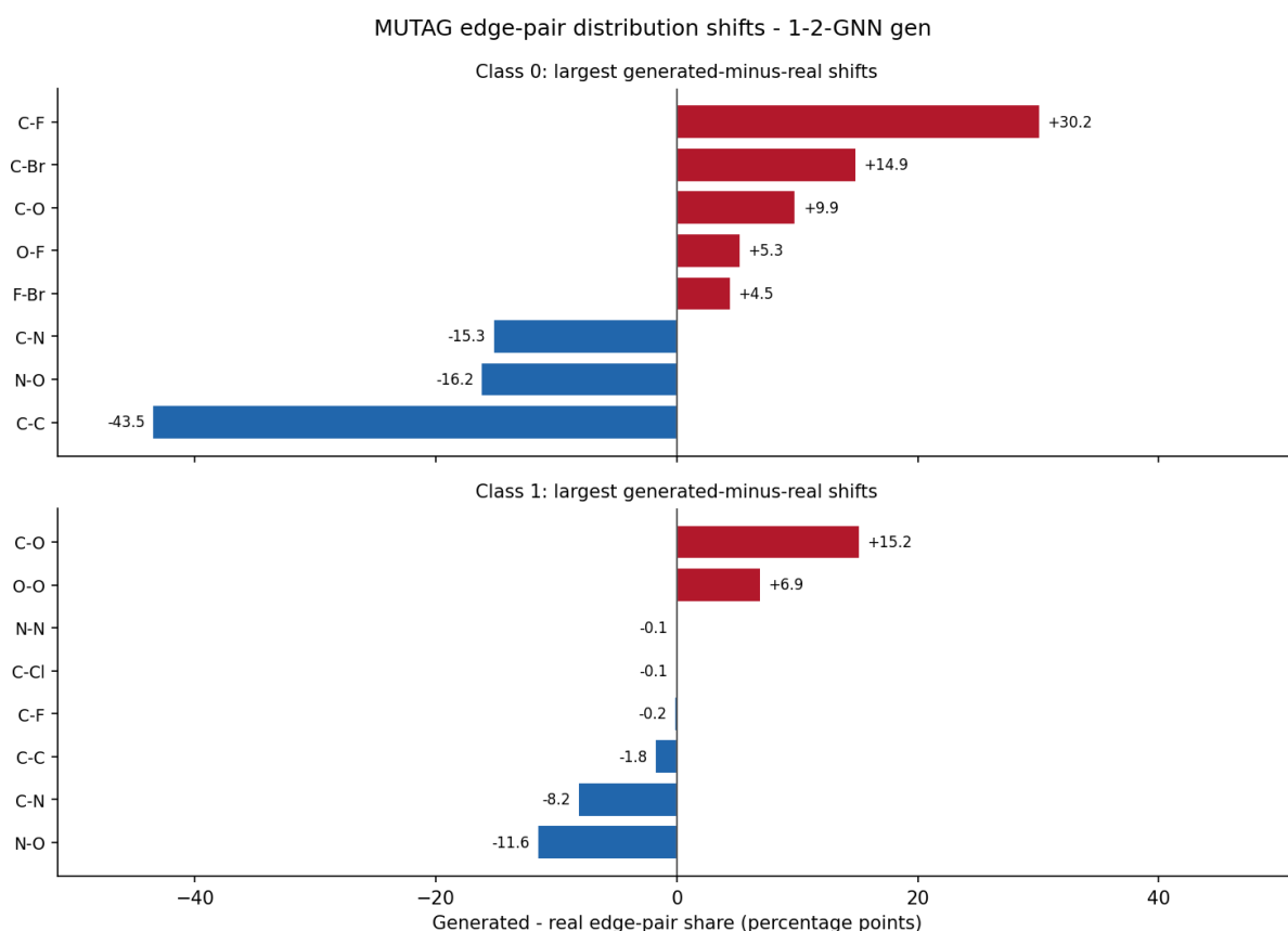
Figure 4: MUTAG edge-type co-occurrence fingerprint for the 1-2-GNN generator. Bars show the largest generated-minus-real changes in unordered atom-pair edge shares, in percentage points, over 1000 generated graphs per class. Positive bars are over-produced by the generator; negative bars are under-produced.
