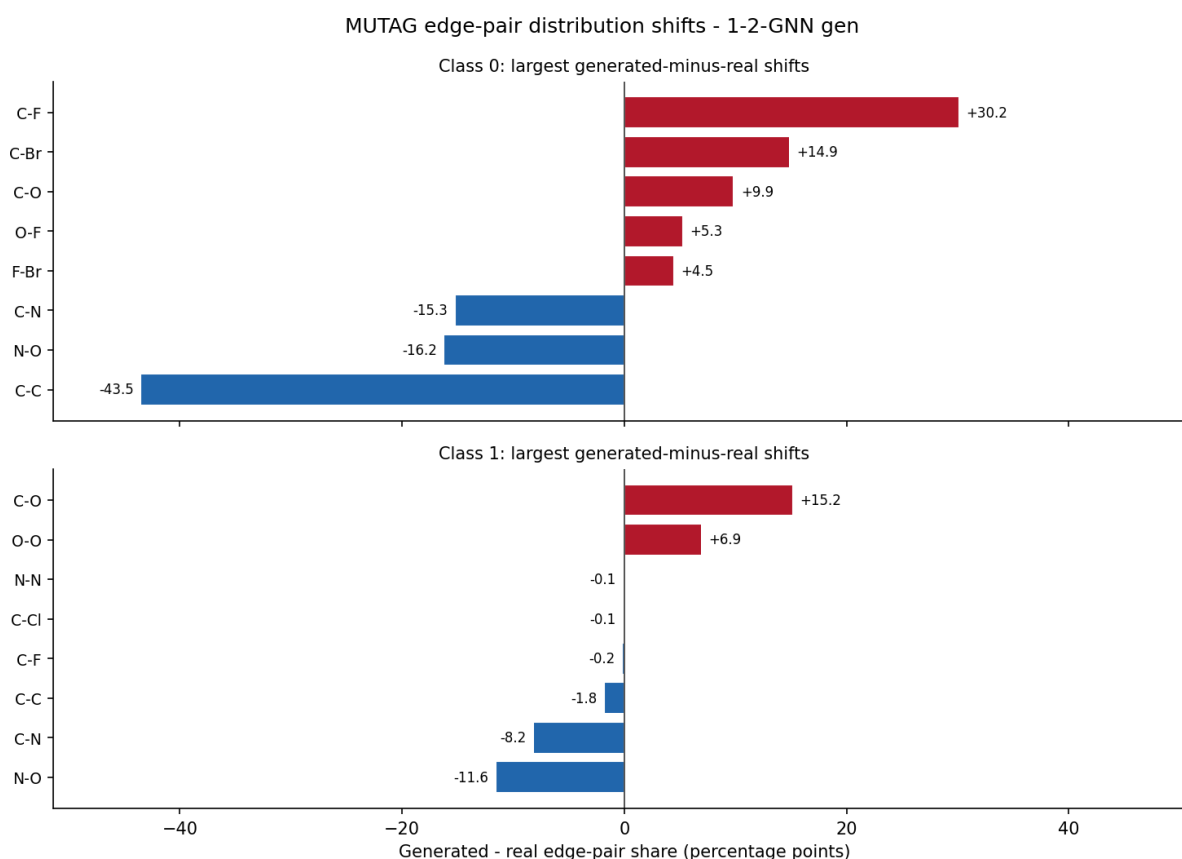
Figure 2: MUTAG edge-type co-occurrence fingerprint for the 1-2-GNN generator. Bars show the largest generated-minus-real changes in unordered atom-pair edge shares, in percentage points, over 1000 generated graphs per class. Positive bars are over-produced by the generator; negative bars are under-produced.
