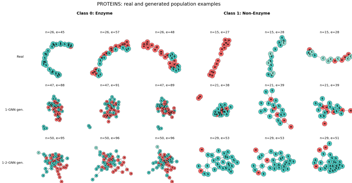
Figure 6: Illustrative PROTEINS examples. Each row shows three median-sized examples from one source: real dataset graphs, the 1-GNN generated population, or the 1-2-GNN generated population. The generated examples make the population-level shifts easier to see, but they are not used as standalone evidence.
