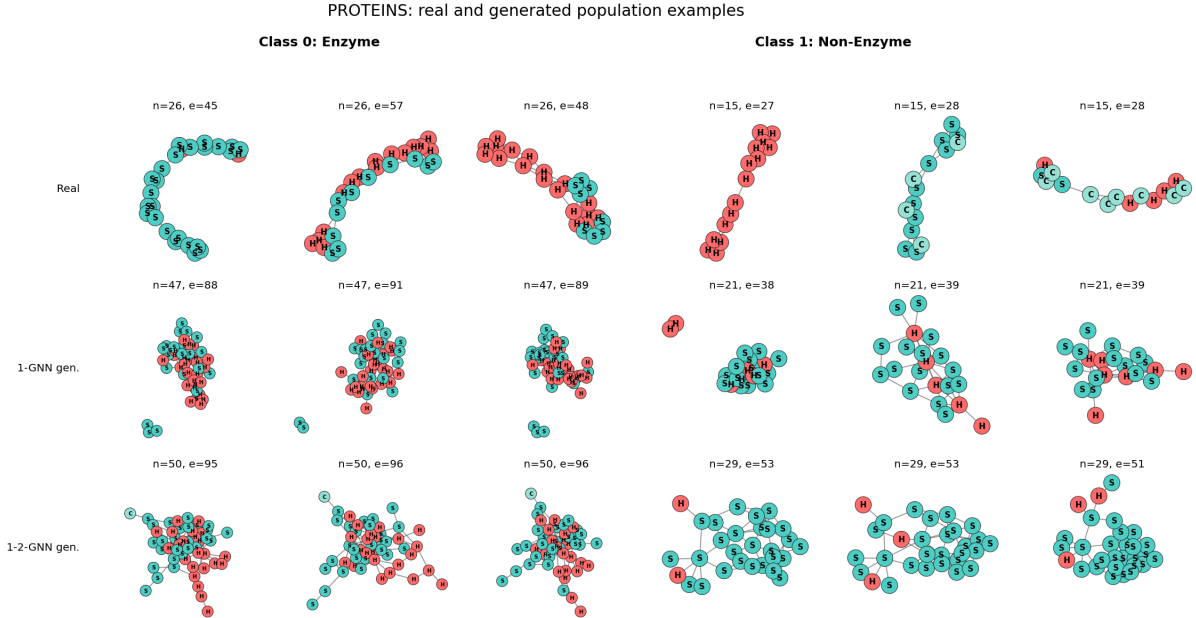
Figure 7: Illustrative PROTEINS examples. Each row shows three median-sized examples from one source: real dataset graphs, the 1-GNN generated population, or the 1-2-GNN generated population. The generated examples make the population-level shifts easier to see, but they are not used as standalone evidence.
