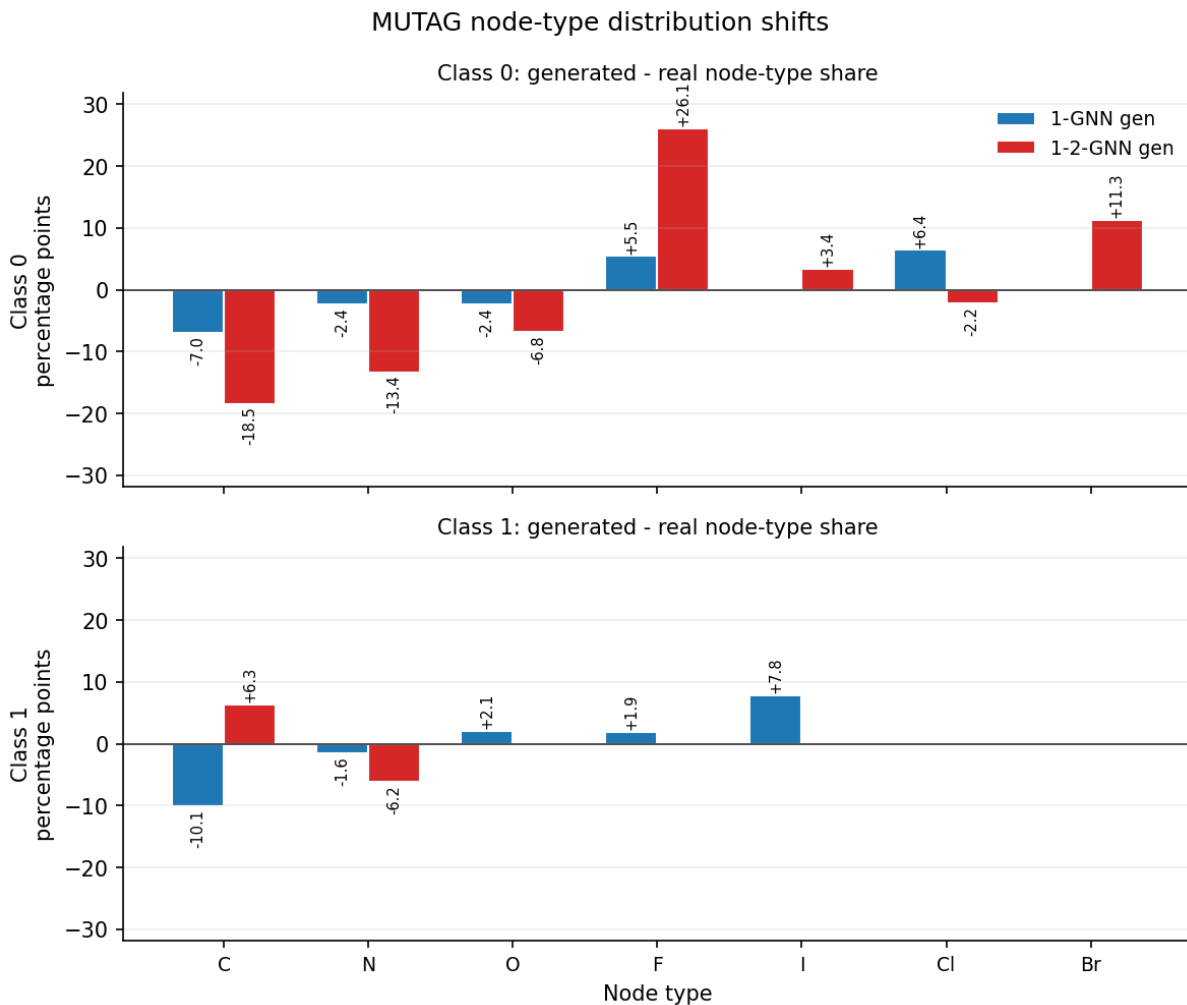
Figure 4: MUTAG atom-type distribution shifts. Bars show generated-minus-real changes in active-node atom shares, in percentage points, over 1000 generated graphs per class. Positive bars are over-produced by the generator; negative bars are under-produced.
