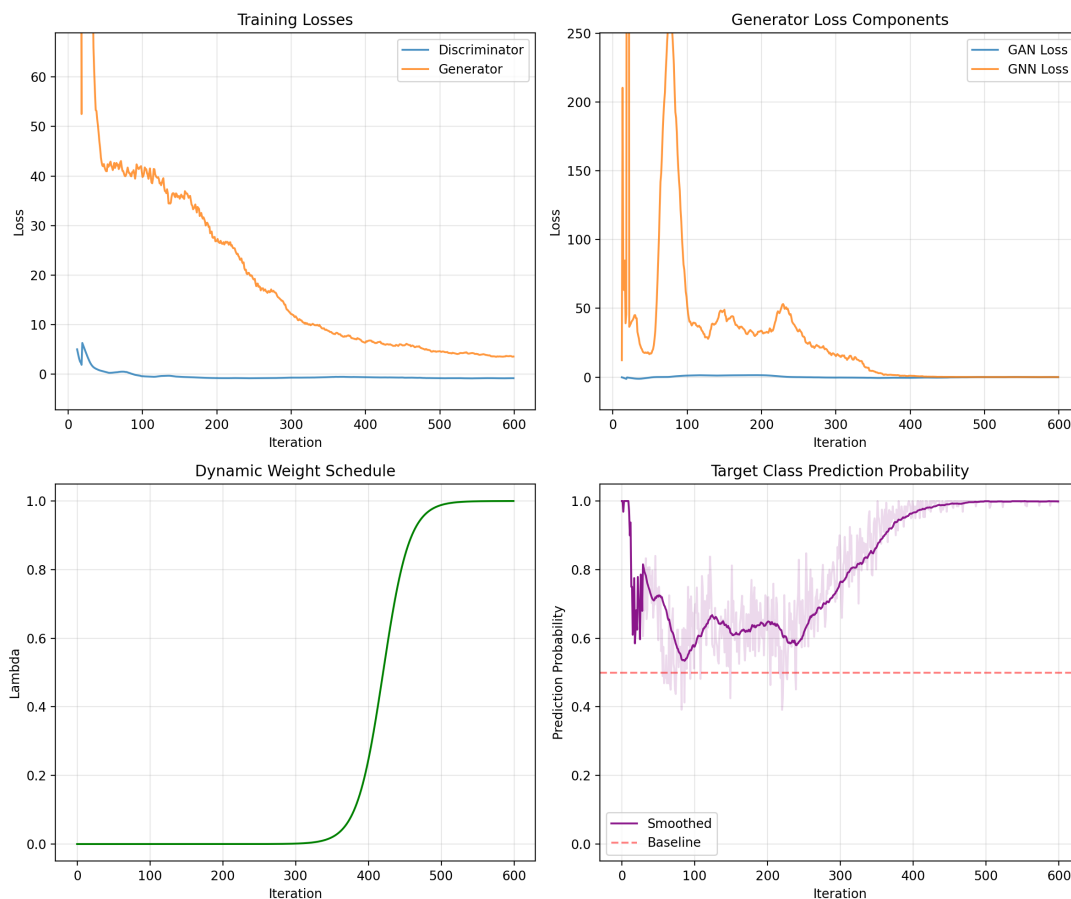
Figure 1: Representative GIN-Graph training history for the MUTAG 1-2-GNN Mutagen generator. The plot is used as a training-dynamics sanity check rather than as proof of monotonic convergence: GAN losses can oscillate because the generator and discriminator co-evolve during training.
