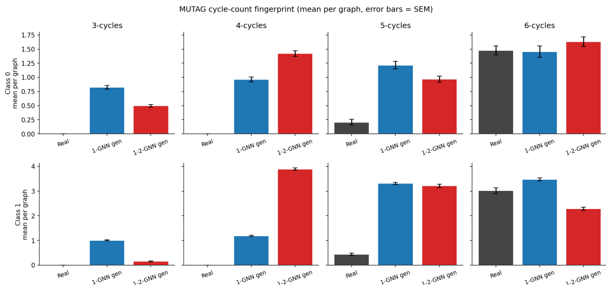
Figure 6: MUTAG simple-cycle counts per graph, aggregated over 1000 generated graphs per cell. Error bars are the standard error of the mean. Real MUTAG has zero 3- and 4-cycles in both classes; both generators introduce them, but the 1-2-GNN’s 3-cycle rate is lower than the 1-GNN’s, while it over-produces 4-cycles.
