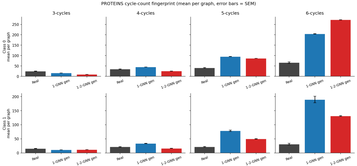
Figure 10: PROTEINS simple-cycle counts per graph, aggregated over 1000 generated graphs per cell. Error bars are the standard error of the mean. Both generators over-produce 5- and 6-cycles relative to real; the strongest differences appear in the 6-cycle panels, with the 1-2-GNN highest in class 0 and the 1-GNN highest in class 1.
