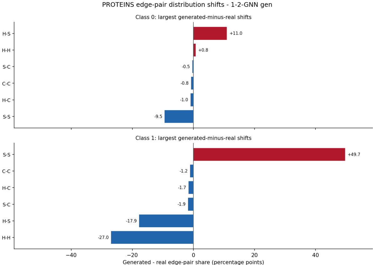
Figure 9: PROTEINS edge-type co-occurrence fingerprint for the 1-2-GNN generator. Bars show the largest generated-minus-real changes in unordered secondary-structure edge-pair shares, in percentage points, over 1000 generated graphs per class. Positive bars are over-produced by the generator; negative bars are under-produced.
