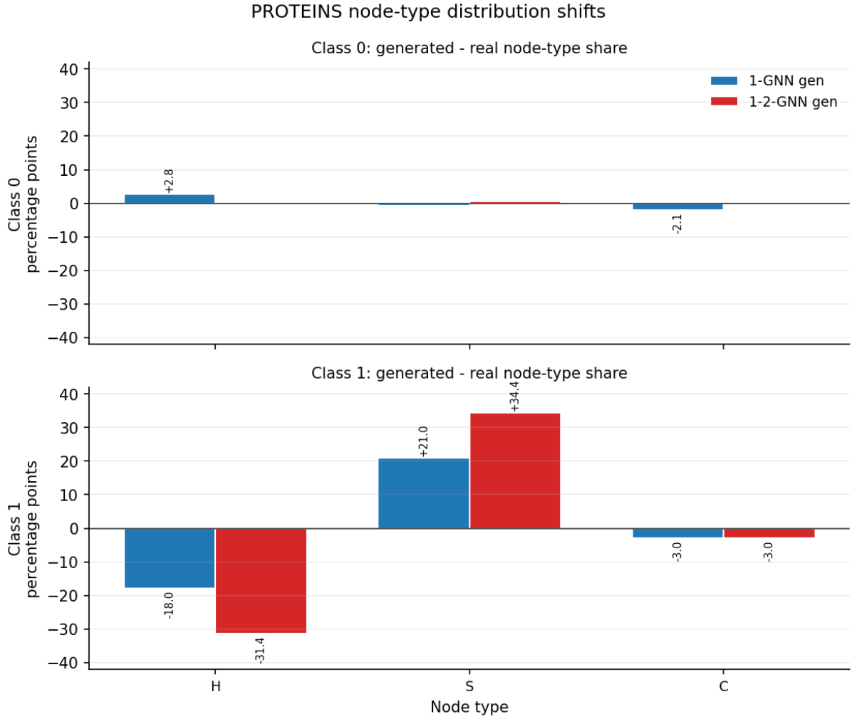
Figure 8: PROTEINS secondary-structure distribution shifts. Bars show generated-minus-real changes in active-node type shares, in percentage points, over 1000 generated graphs per class. Here H denotes Helix, S denotes Sheet, and C denotes Coil/Turn.
