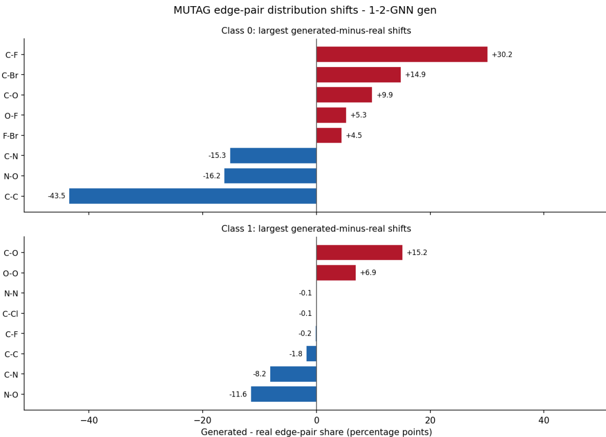
Figure 5: MUTAG edge-type co-occurrence fingerprint for the 1-2-GNN generator. Bars show the largest generated-minus-real changes in unordered atom-pair edge shares, in percentage points, over 1000 generated graphs per class. Positive bars are over-produced by the generator; negative bars are under-produced.
