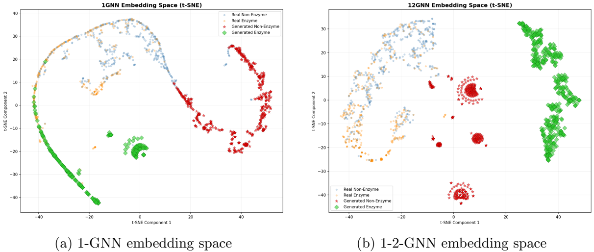
Figure 8: t-SNE projections of PROTEINS real (small dots) and generated (large markers) graph embeddings. Colours distinguish Non-Enzyme (class 0) from Enzyme (class 1).
