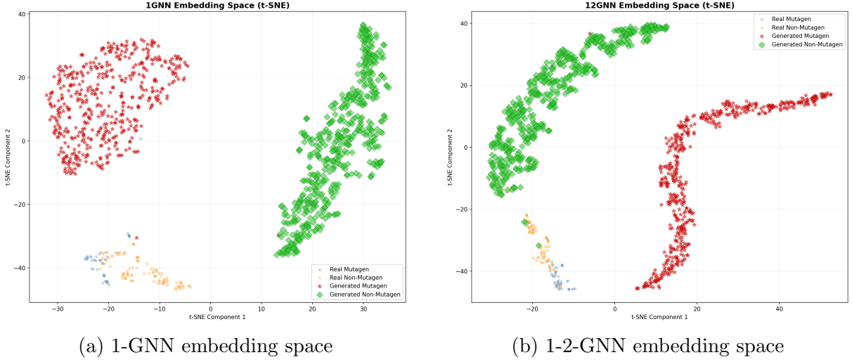
Figure 7: t-SNE projections of MUTAG real (small dots) and generated (large markers) graph embeddings. Colours distinguish Mutagen (class 0) from Non-Mutagen (class 1).
