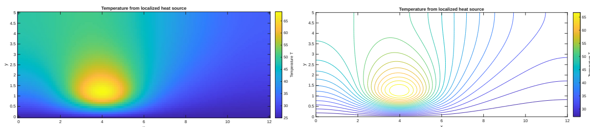
Figure 11: Image and contour plots for h = 0.1 . The hottest area is close to the source at (4, 1) .
