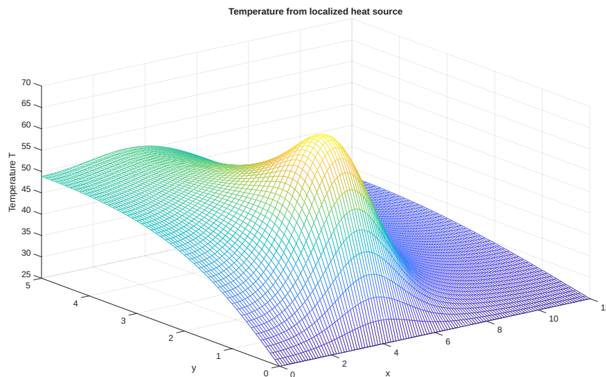
Figure 10: Mesh plot for the localized source with h = 0.1 .
