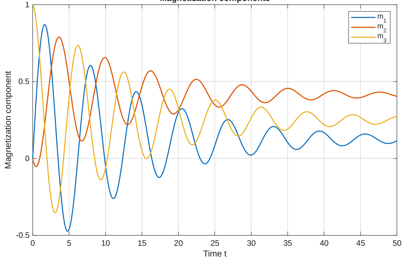
Magnetization components
