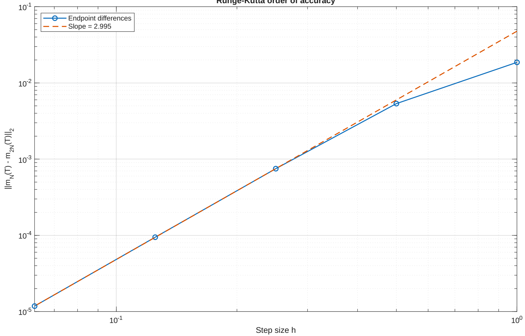
Runge-Kutta order of accuracy
