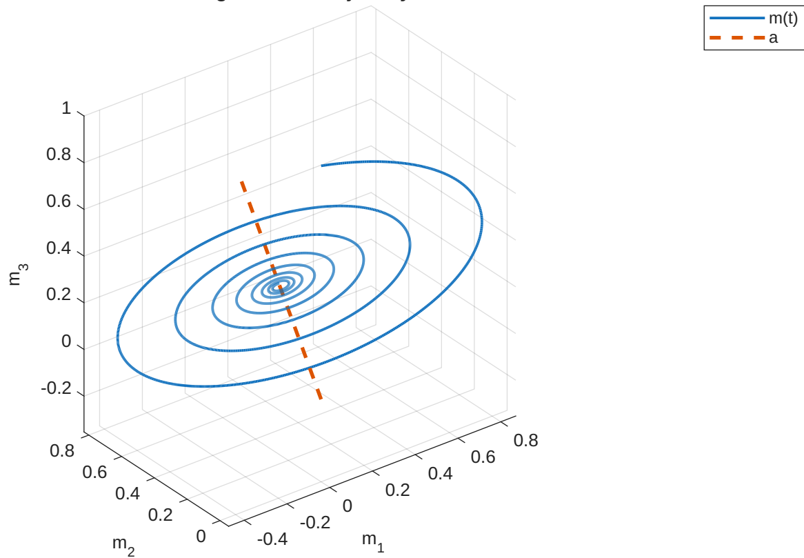
Magnetization trajectory
