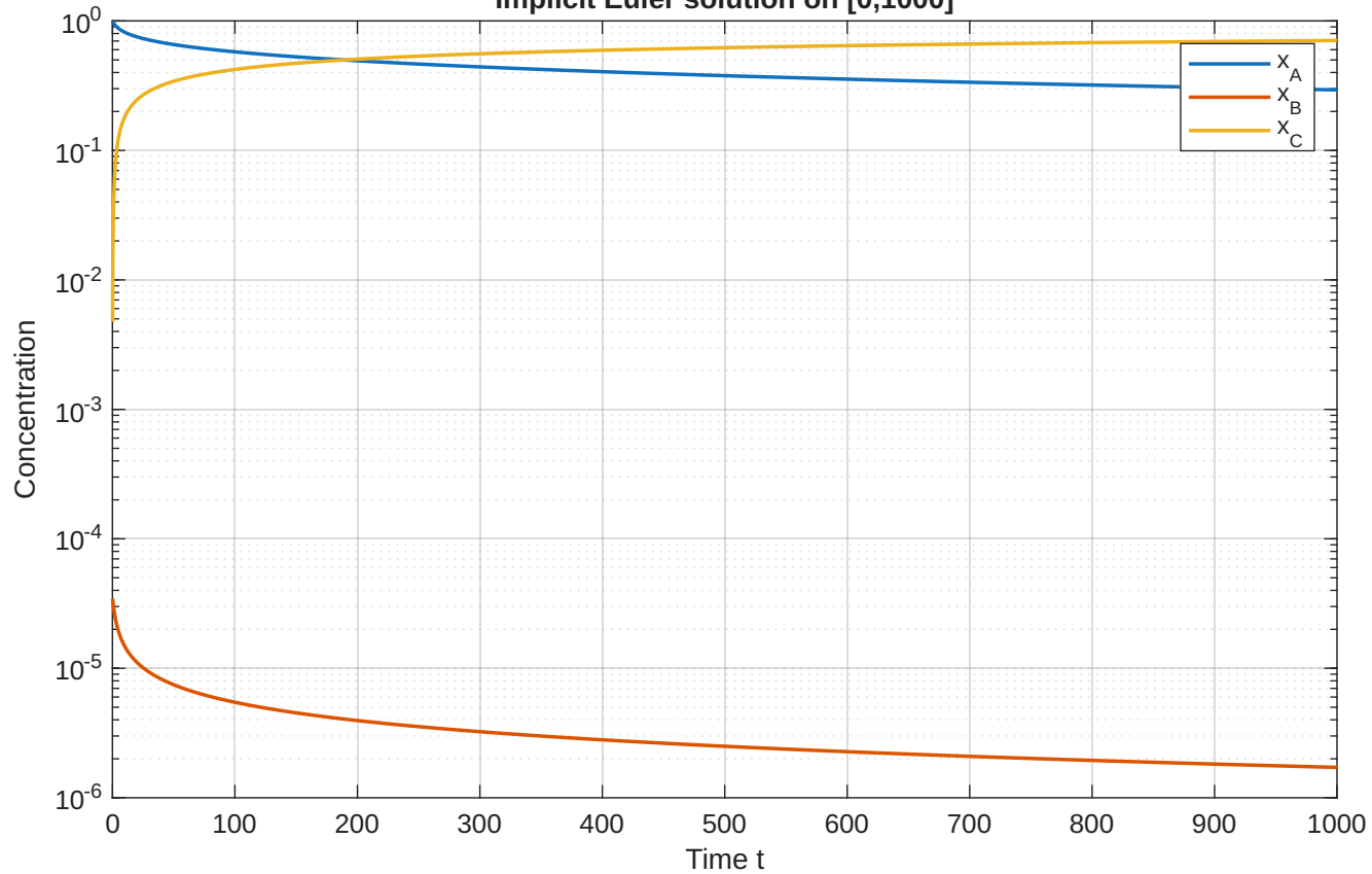
Implicit Euler solution on [0,1000]
