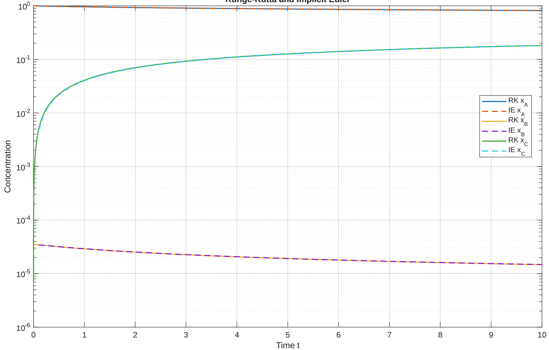
Runge-Kutta and Implicit Euler
