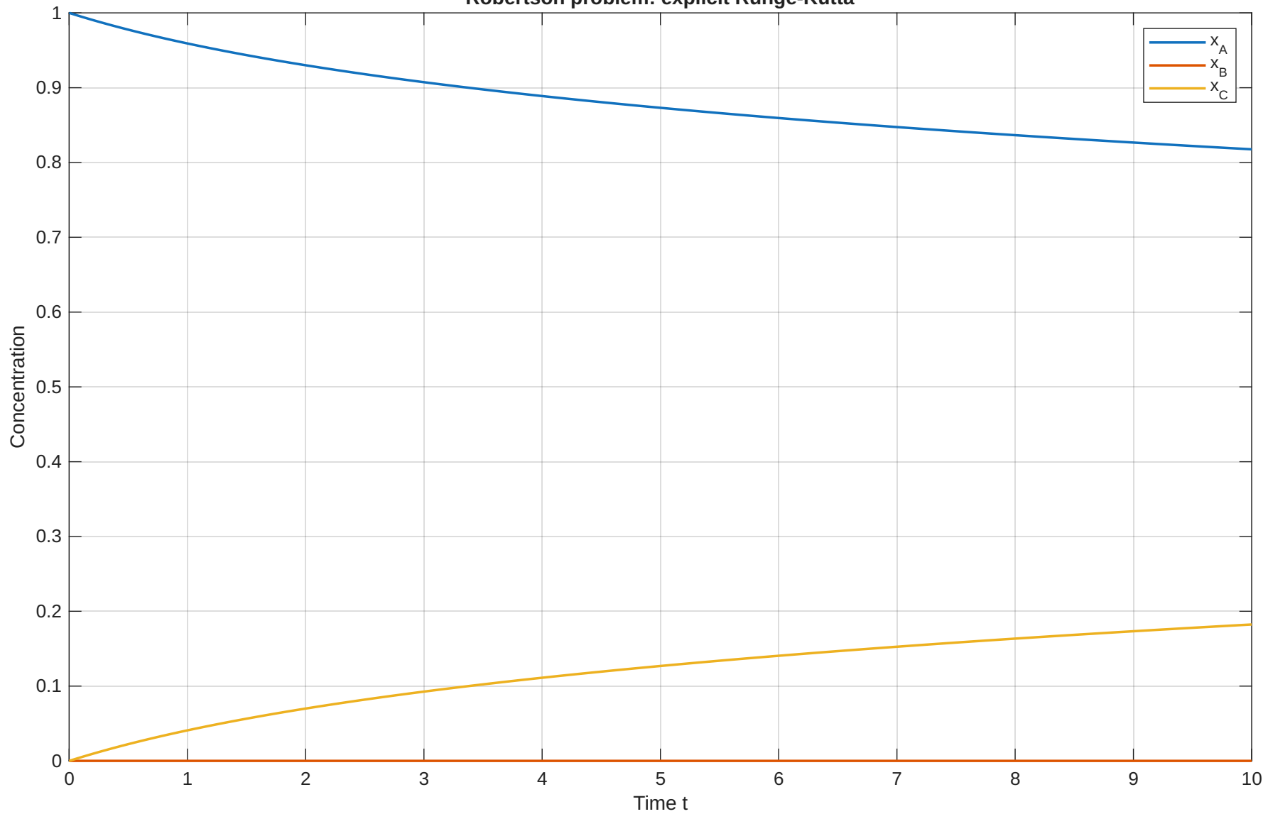
Robertson problem: explicit Runge-Kutta
