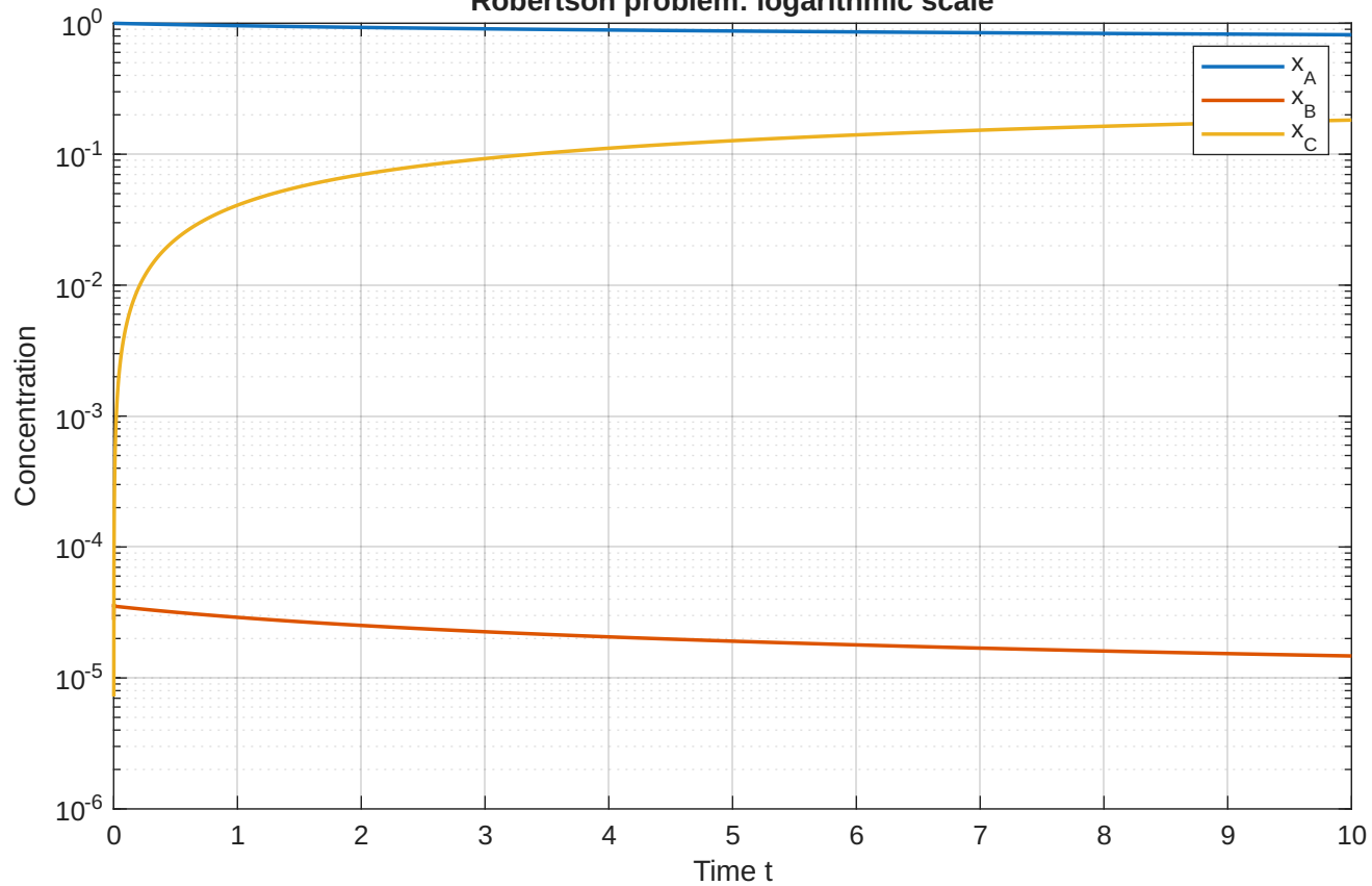
Robertson problem: logarithmic scale
