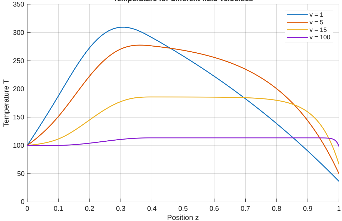
Temperature for different fluid velocities
