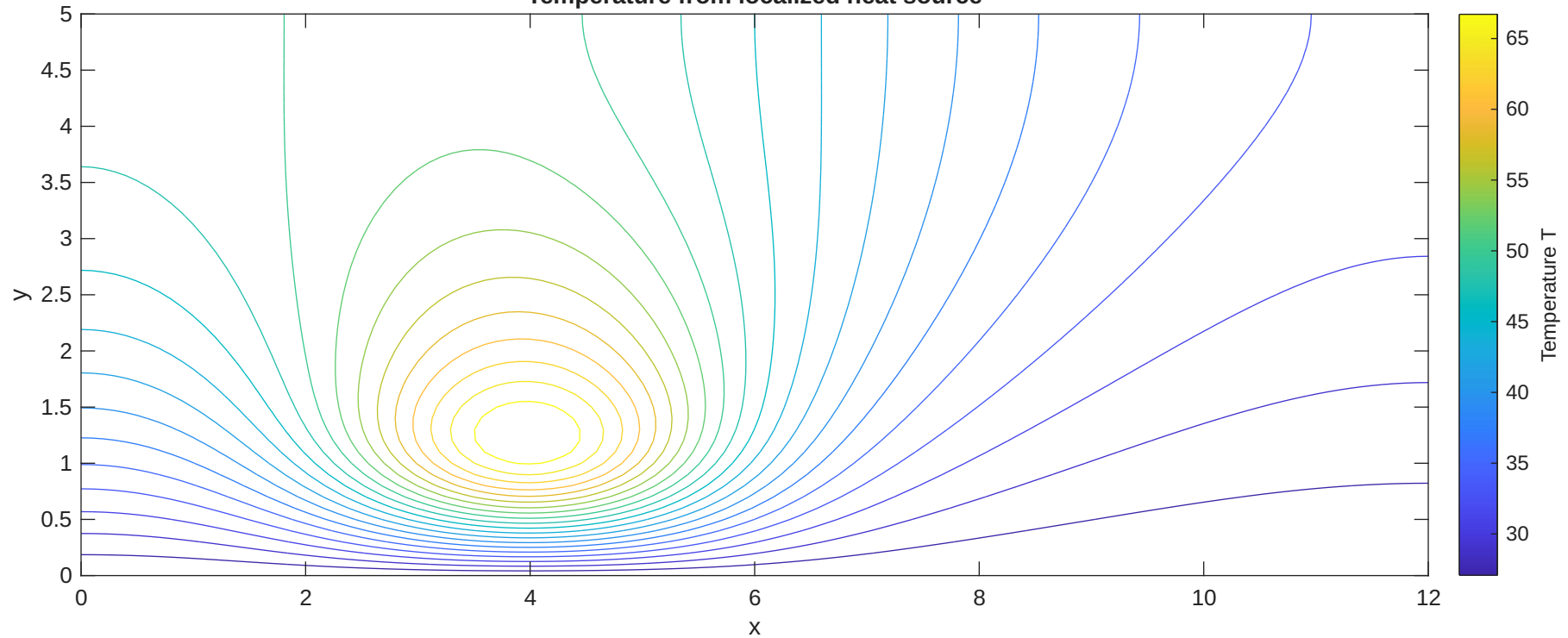
Temperature from localized heat source
