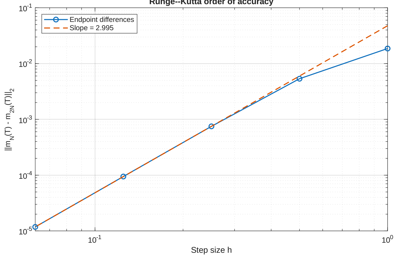
Runge--Kutta order of accuracy
