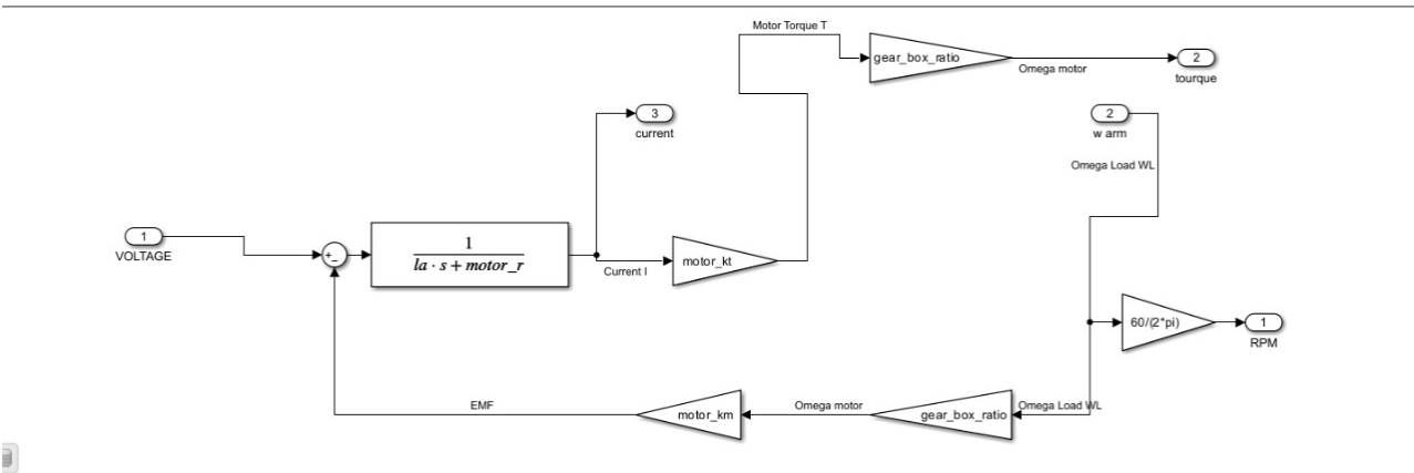
Figure 15 motor model for simulation
