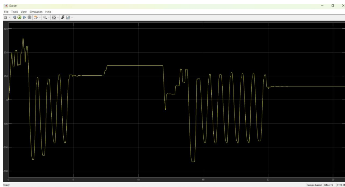
Figure 22 motor angular velocity
