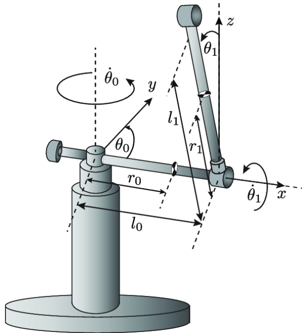
Figure 1 furuta pendulum
