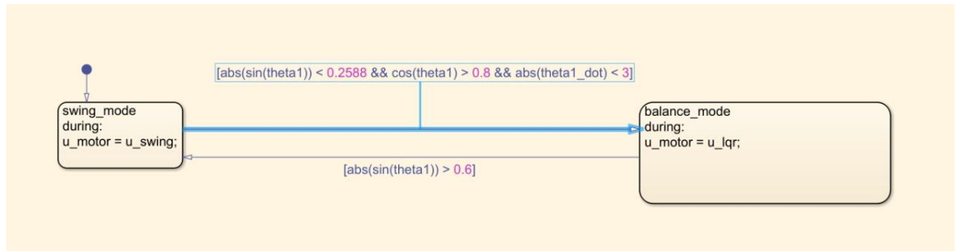
Figure 17 stateflow chart for simulations
