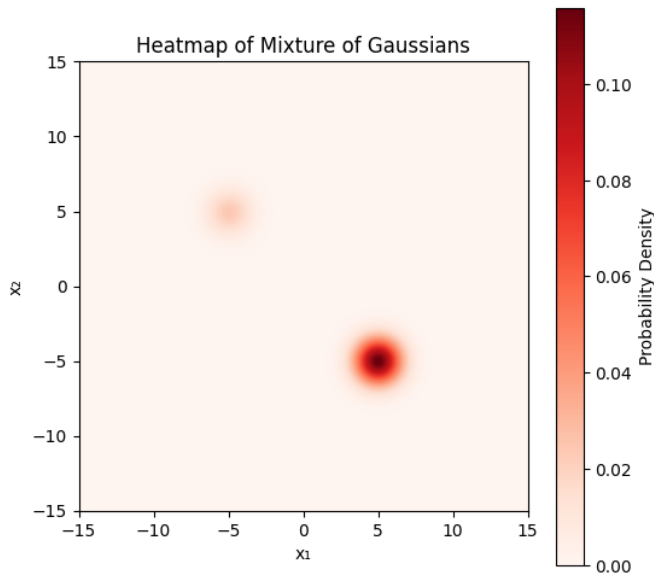
Figure 1: True probability density heatmap of 2D Gaussian mixture
