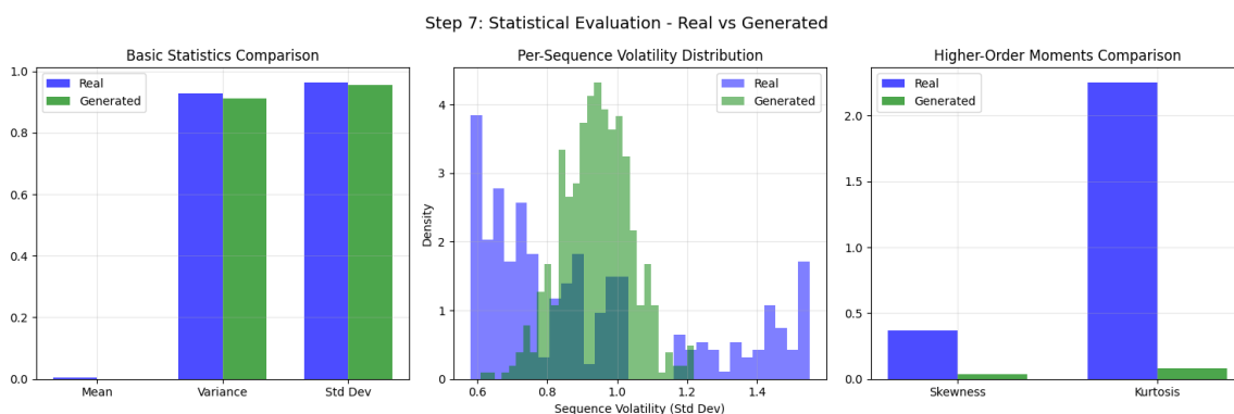
Figure 15: Statistical Metrics Comparison. Left: Mean/Variance. Middle: Volatility Distribution. Right: Higher-Order Moments.
