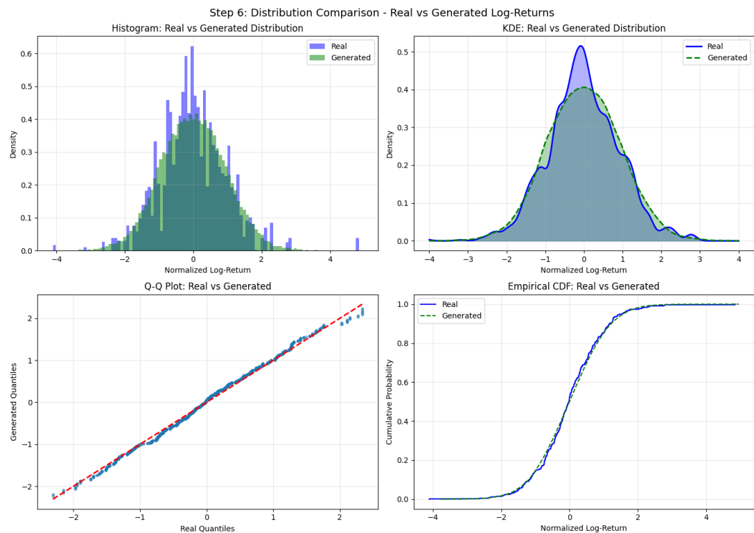
Figure 32: Step 6: Distribution Comparison - Histogram KDE (Cell 71, Output 2)
