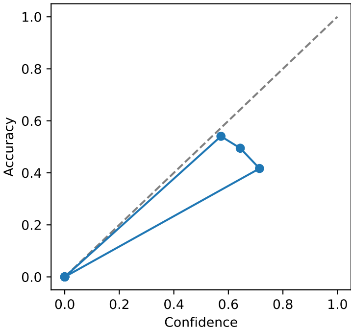
Reliability (ECE=0.145)
