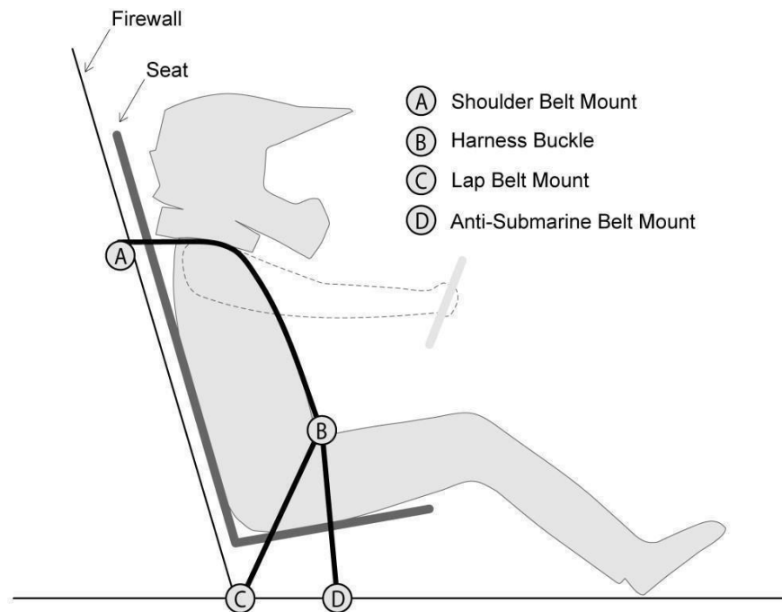
Figure B-25: Driver Harness Schematic
