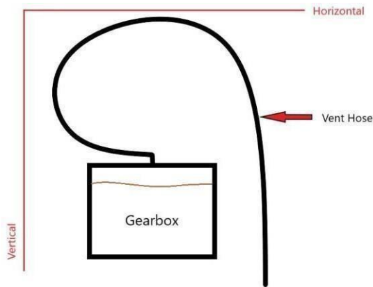
Figure B-52: Air Trap Vent Line Routing
