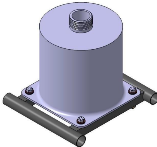
Figure B-41: Fuel tank mounted to square/rectangular tubes (preferred mounting design)
