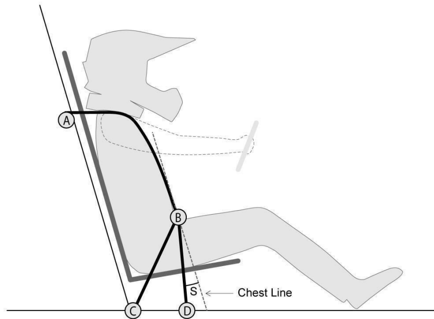
Figure B-33: Driver Harness, Anti-Submarine Belt Angle
