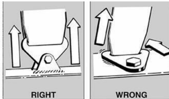
Figure B-32: Driver Harness, Lap Belt Tab Orientation
