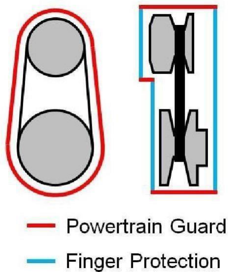
Figure B-50: Powertrain Guard Extent example on a CVT
