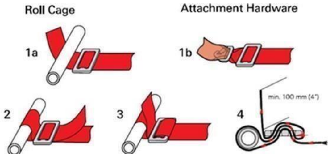
Figure B-30: Driver Harness, Diagram of Proper Wrapping of Webbing
