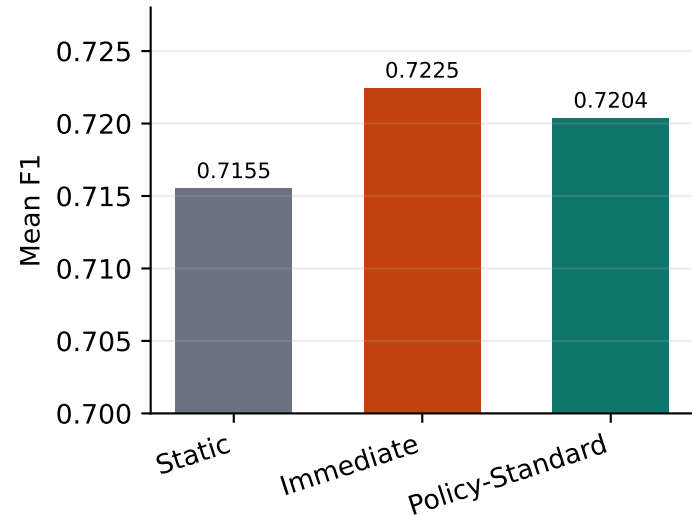
Predictive Performance
