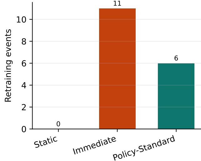
Adaptation Cost
