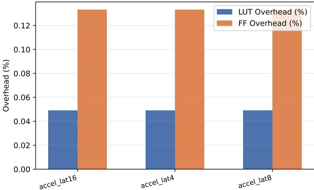
Adapter Resource Overhead (Shell baseline: 67K LUTs)
