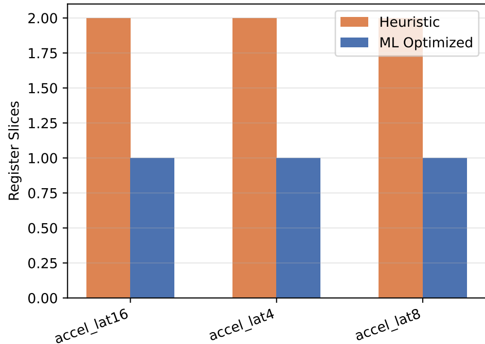
Register Slices: ML vs Heuristic
