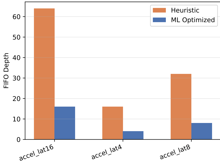
FIFO Depth: ML vs Heuristic
