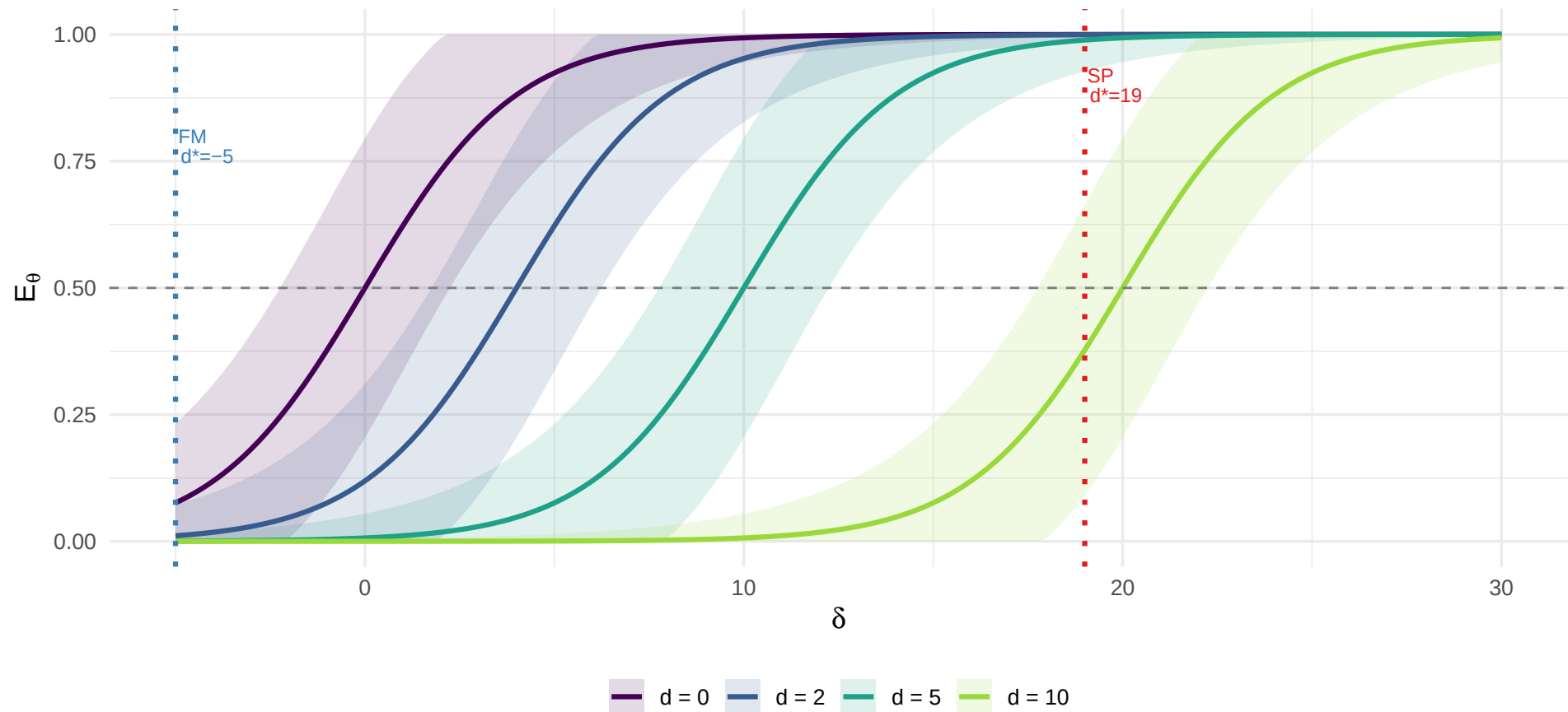
Attack Success Probability vs delta, by Defense Level
