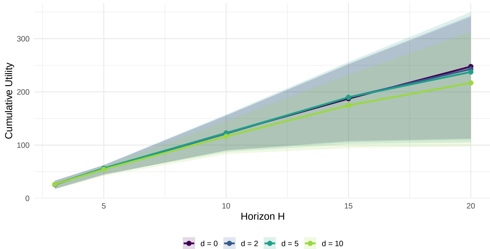
Cumulative Attacker Utility vs Horizon H (FM)
