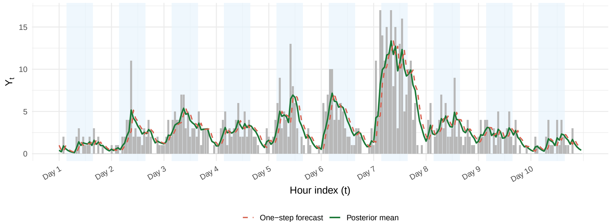
Avazu Hourly Click Counts and PGSS Filter
