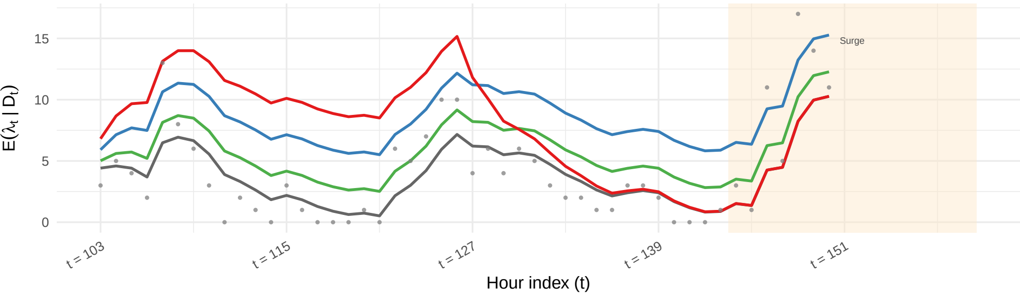
Sequential Click-Fraud Attack: Filter Trajectory and Forecast Inflation
