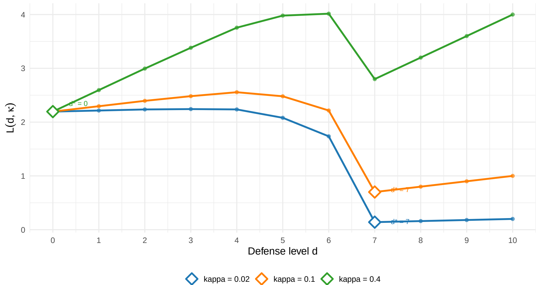
Defender Loss Surface: L(d; \kappa) = E[KL \mid d] + \kappa * d
