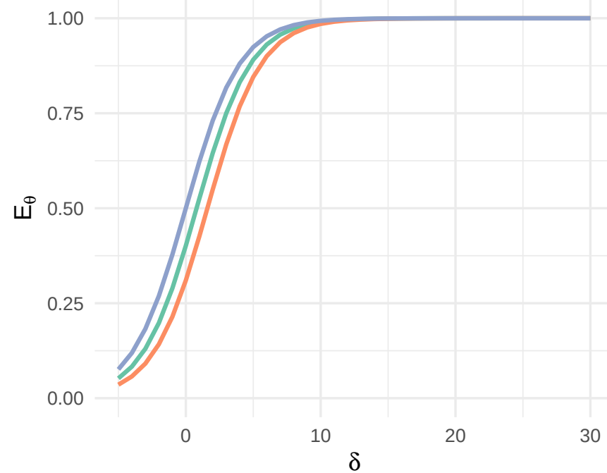
Vary s_2 (deterrence)
