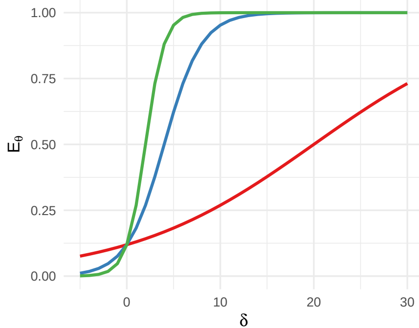
Vary s_1 (sensitivity to \delta )
