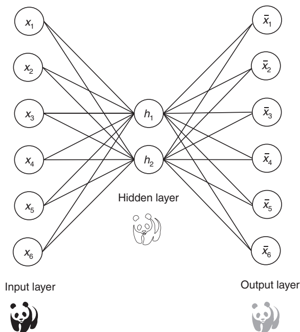
FIGURE 4.1 Lossy compression.
