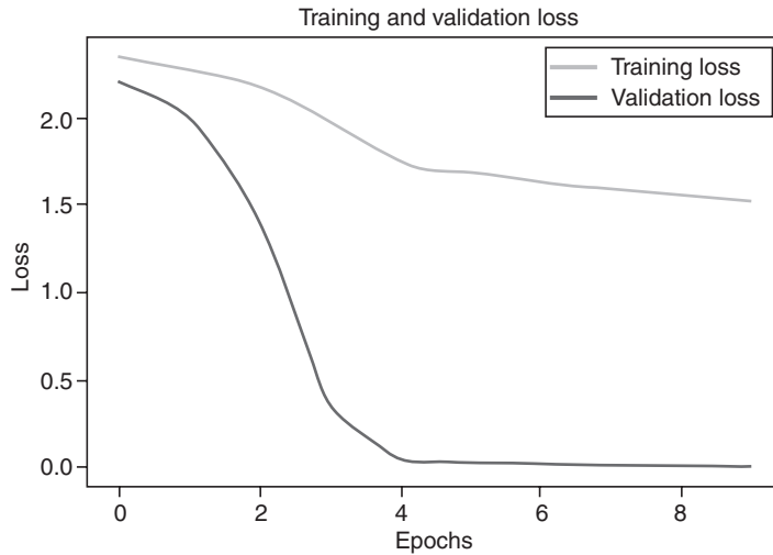
FIGURE 7.8 Loss graph.
