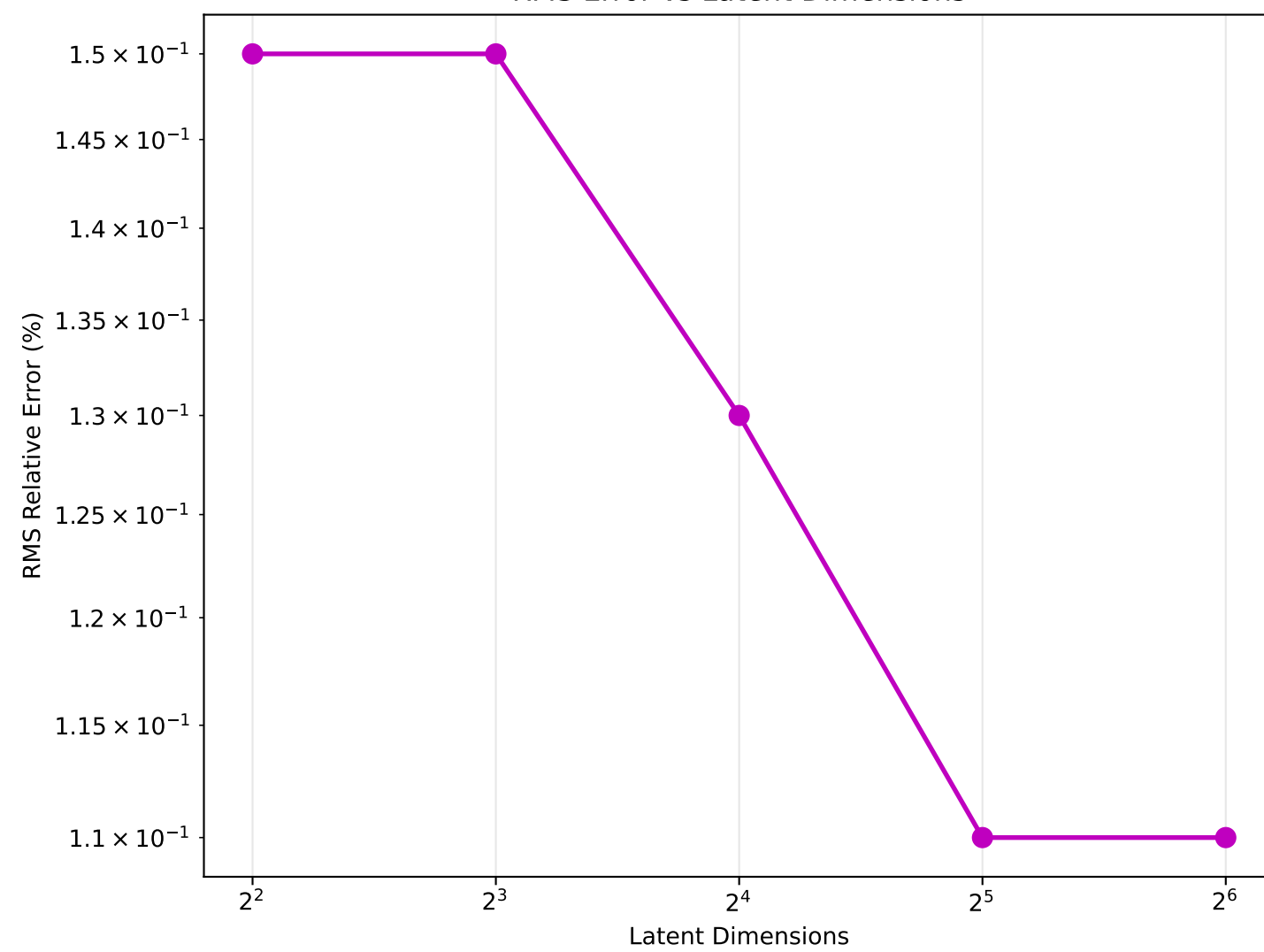
RMS Error vs Latent Dimensions
