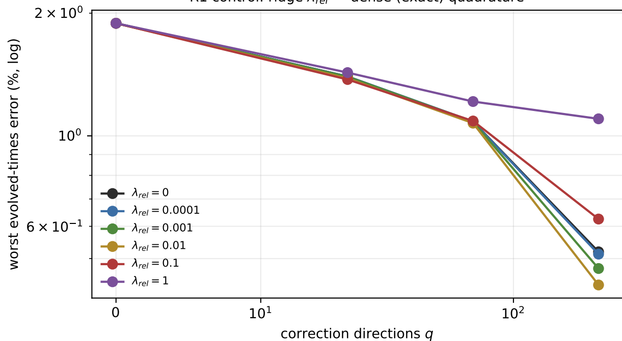
R1 control: ridge \lambda_{rel} — dense (exact) quadrature
