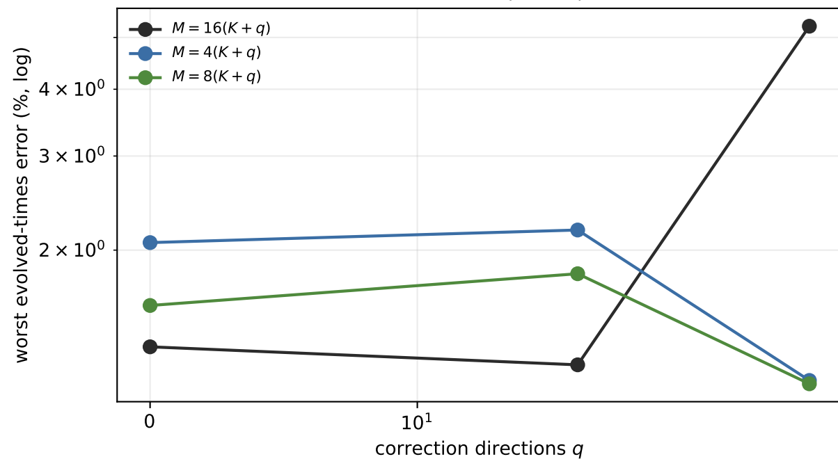
R2 control: test-count rule — empirical quadrature, m = 4M
