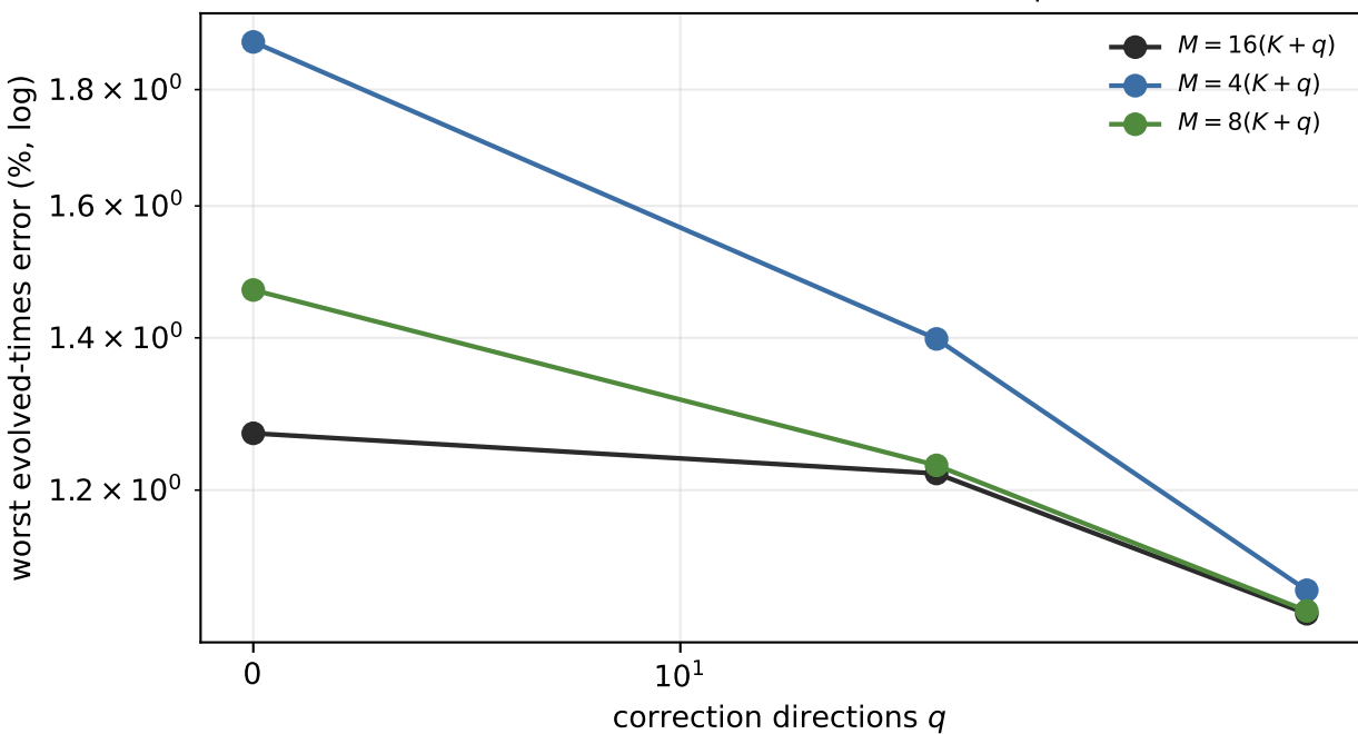
R2 control: test-count rule — dense (exact) quadrature
