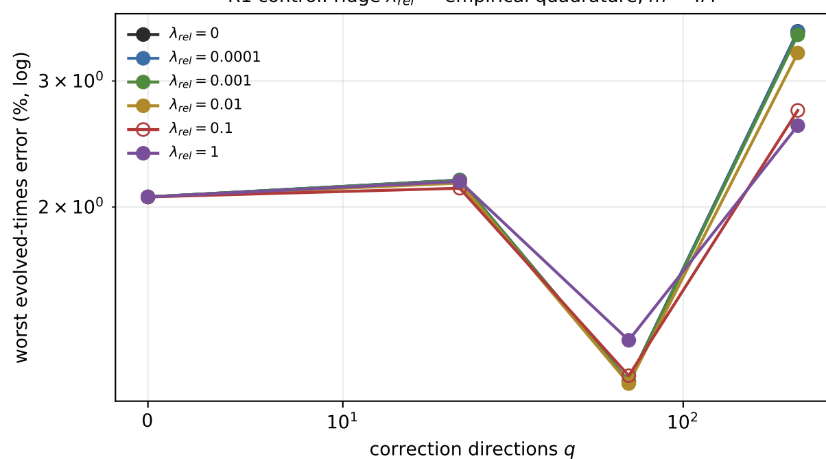
R1 control: ridge \lambda_{rel} — empirical quadrature, m = 4M
