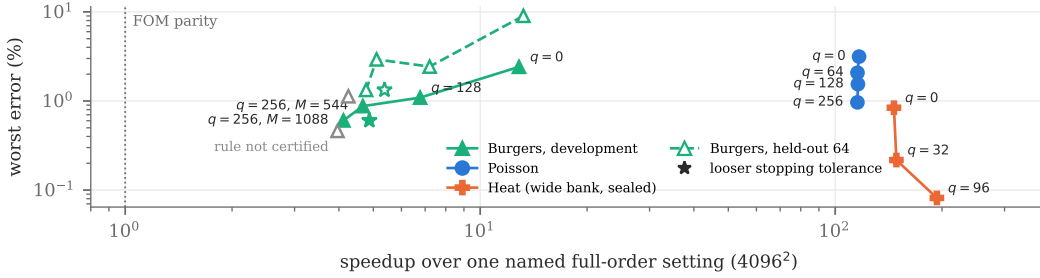
Figure 2: Worst error (evolved times for Burgers and heat) against speed at 4096 2 ; one frozen model and allocation per series, each divided by one full-order setting, the fastest at least as accurate as its best point (Newton–BiCGStab tolerance 3 \times 10^{-3} ; CN–CG \Delta t = 0.025 , \text{rtol } 10^{-6} ; CG \text{rtol } 10^{-1} ). On Burgers q and M change together ( M \approx 4(k + q) , M = 544 an alternative at q = 256 ; fixed- M ladder: Table C.8). Star: looser stopping tolerance; grey: rule failed its held-out check.
