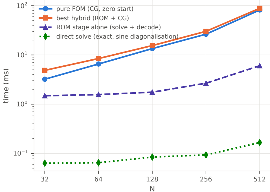
Poisson-2D cost vs mesh ( \tau_{FOM}=1e-10 )
