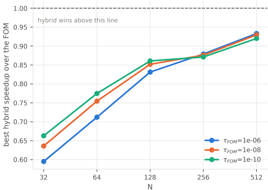
Does the hybrid ever win? No: best 0.933x
