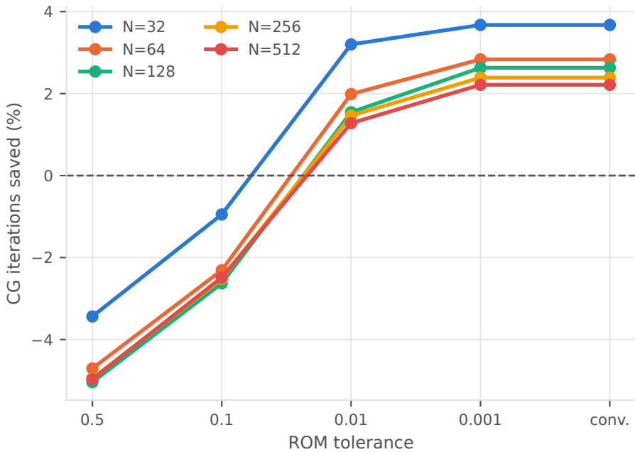
CG iterations saved by the warm start ( \tau_{FOM}=1e-10 )
