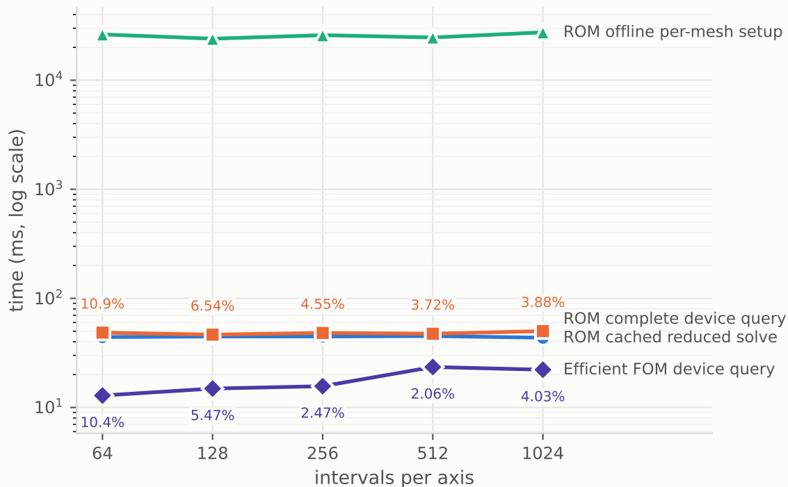
Burgers 2D
