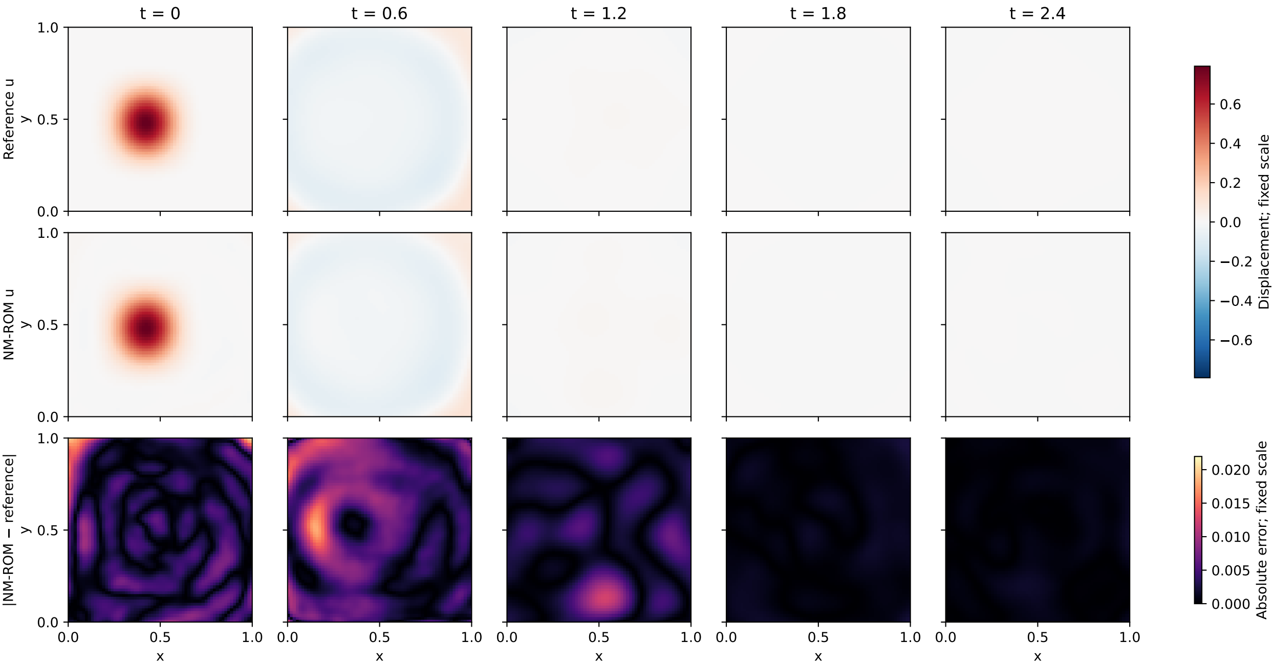
Absorbing wave evolution — development case 1 ROM solves at 512 intervals; display at 64; frozen weights
