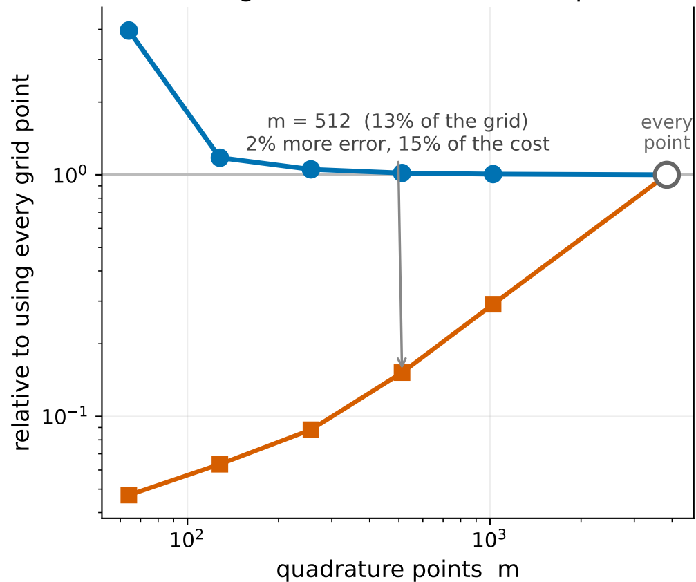
Burgers (cost = one time step)
