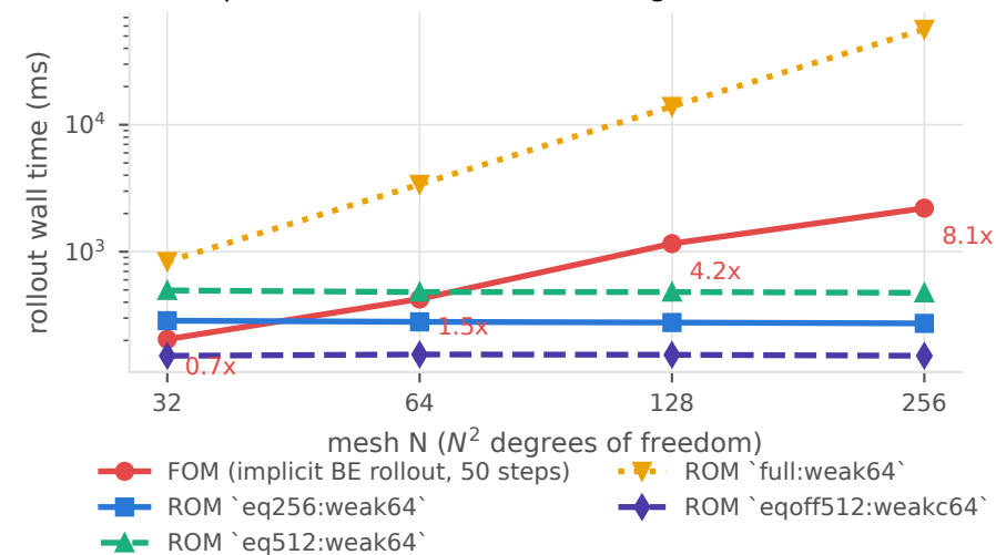
50-step rollout: ROM flat, FOM rising
