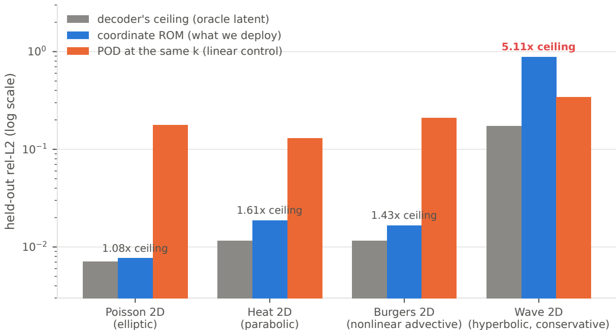
All four PDEs at k = 8 , N = 64 : the ROM reaches the decoder's ceiling — except on Wave
