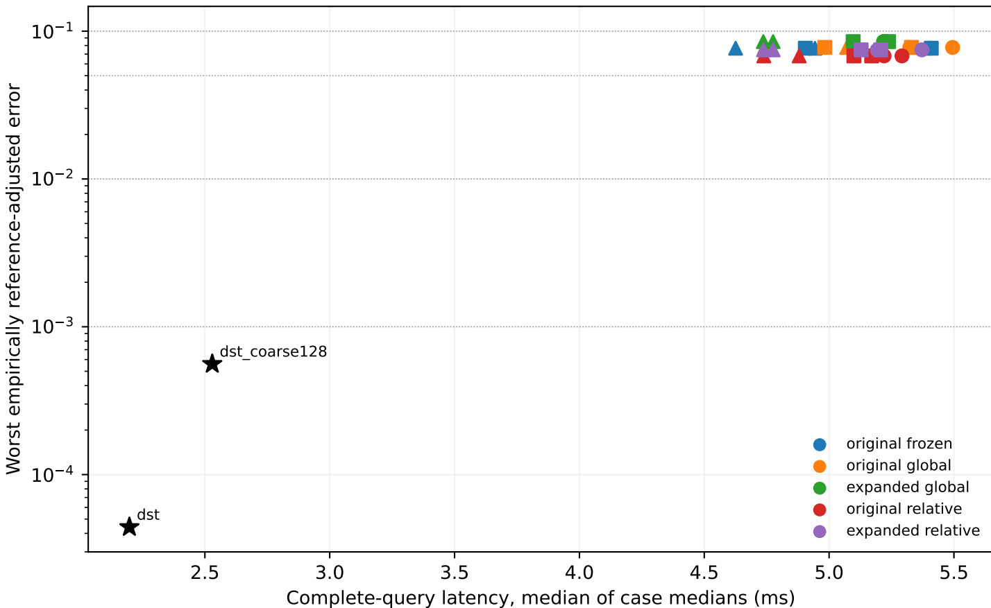
Poisson development cost and error, 512 intervals Circle: modular; square: fused; triangle: guarded kernel; hollow: invalid
