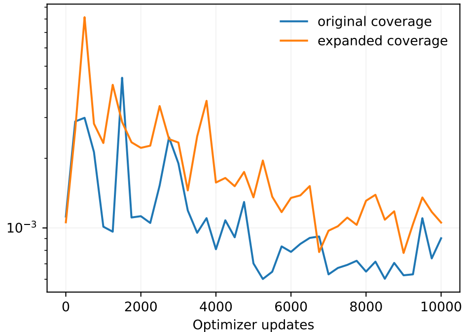
Relative normalization
