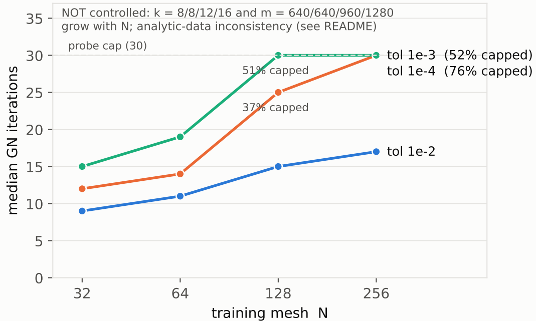
(b) Poisson: iters per cold-start solve (shipped configs)
