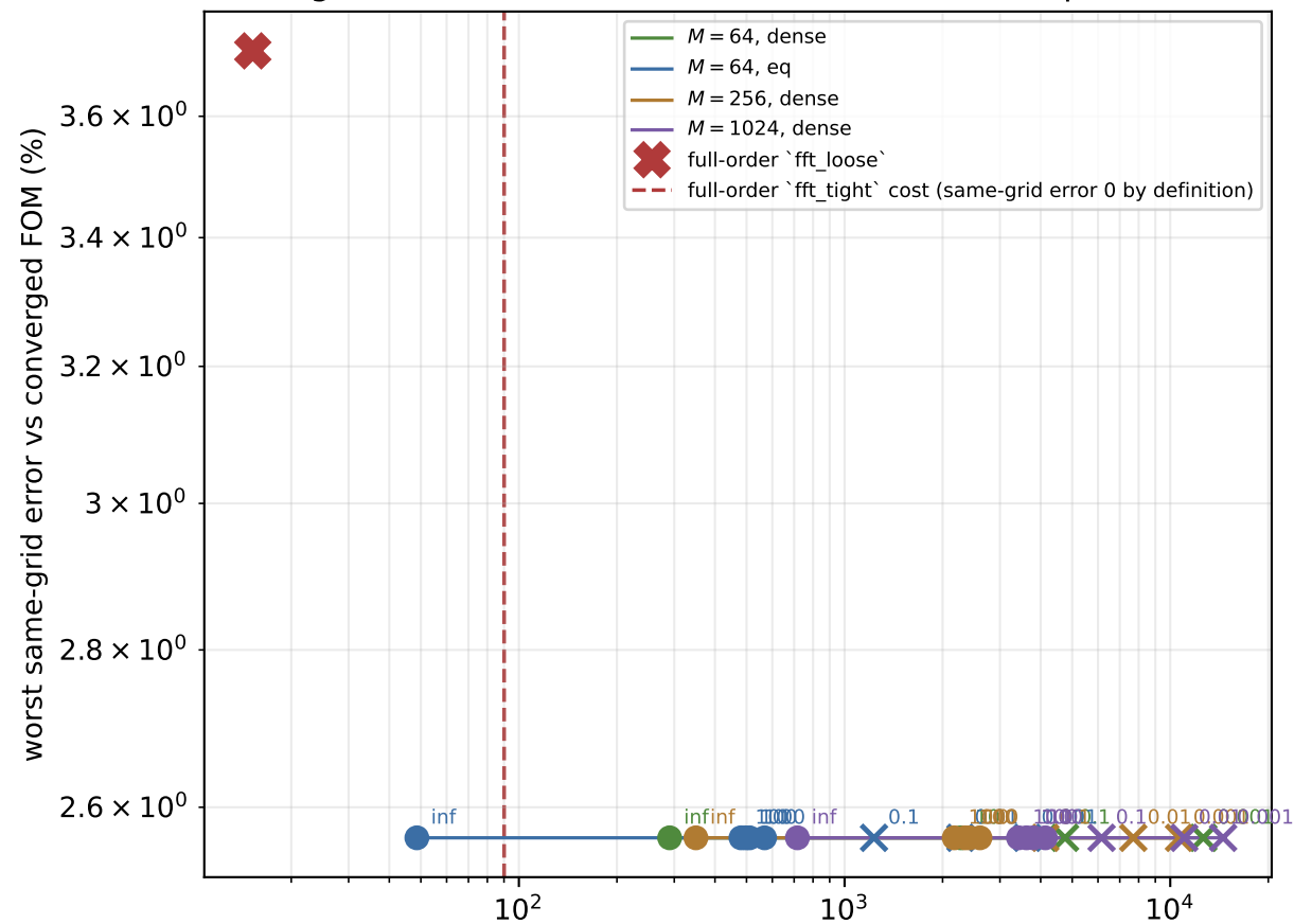
Burgers 2D, 256 intervals: worst over all six output times
