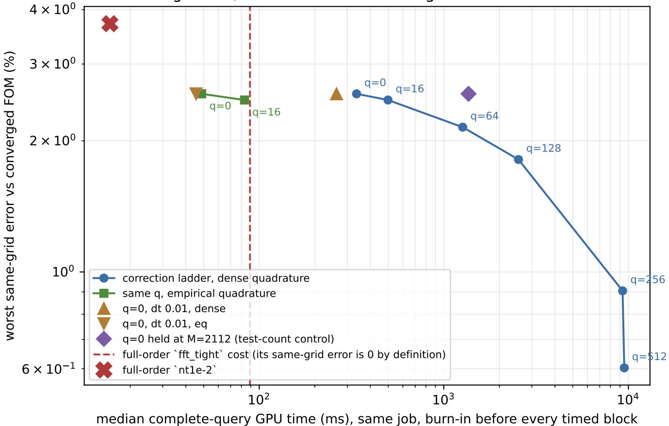
Burgers 2D, 256 intervals: fixed-weight correction ladder
