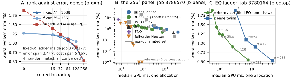
Figure 1: Burgers accuracy and cost. A: correction rank at fixed and scheduled test counts; no cross-job timing ratio is formed. B: paired GPU runtime and worst evolved error, with the non-dominated set marked. C: empirical quadrature against dense residual evaluation. Construction-level confirmation is restricted to q = 0, 16, 32 ; higher-rank qualifications are given in Appendix G.2.
